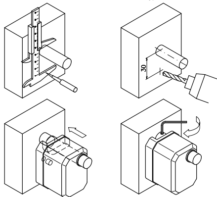
Fig. 1: Mounting instructions
